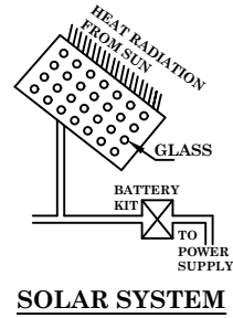
SOLAR SYSTEM
