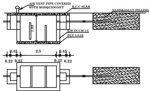
PLAN&SECTION OF SEPTIC TANK TRENCH
