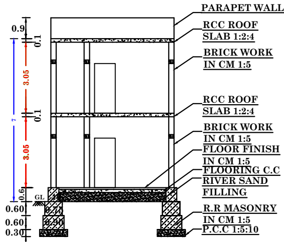
SECTION ON AA1
