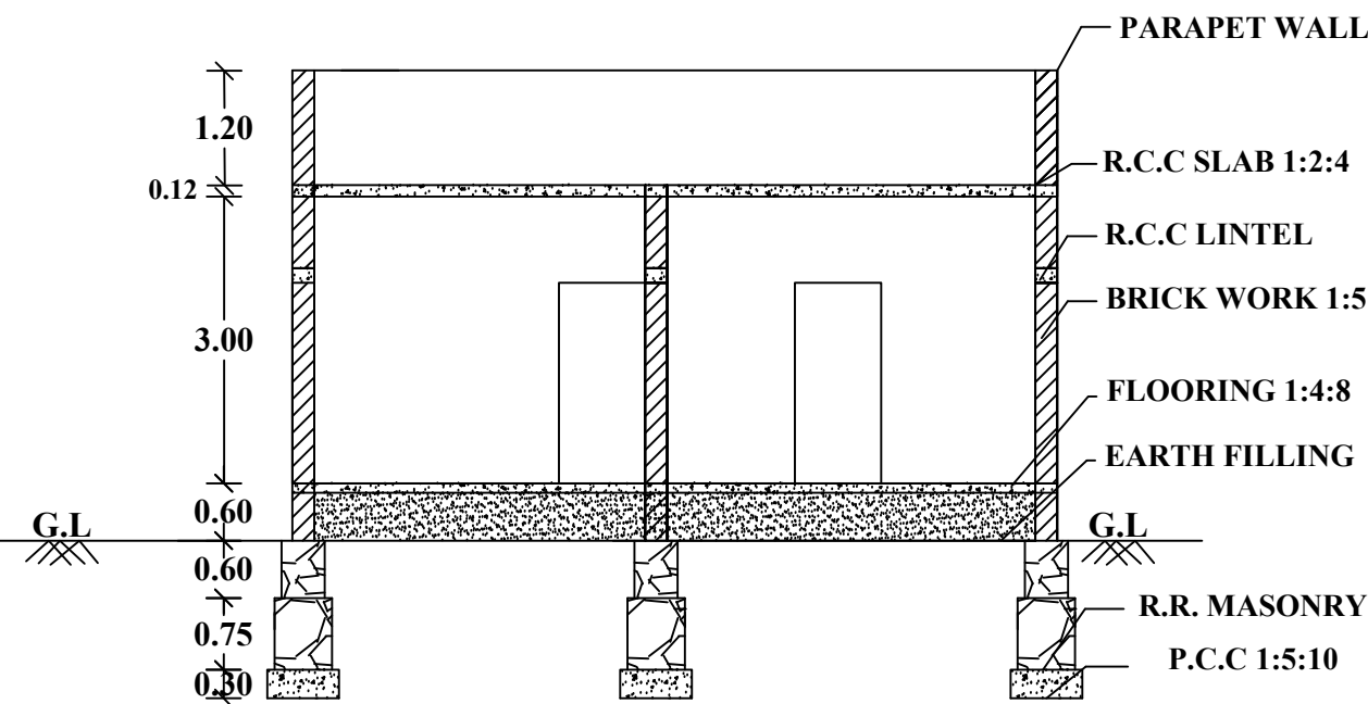
SECTION "AB"
