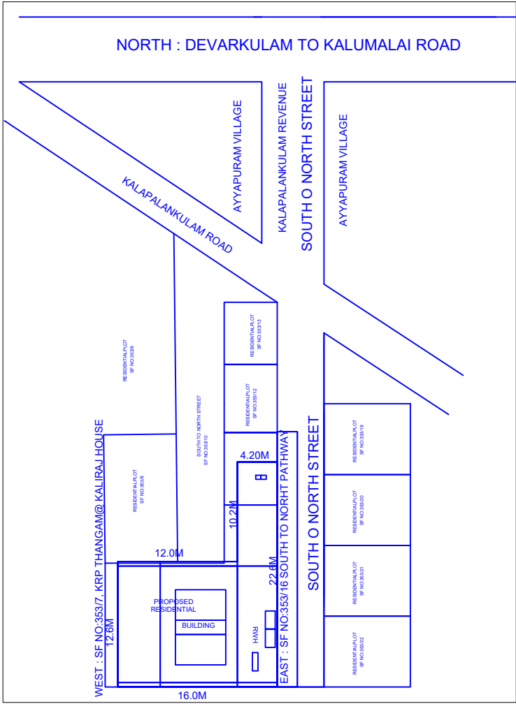
LOCATION PLAN SCALE 1:400
