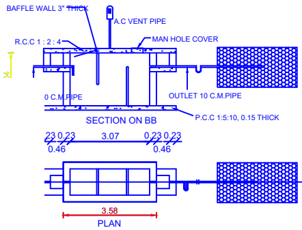
TIC TANK AND TRENCH & U TRAP ADOPTED
