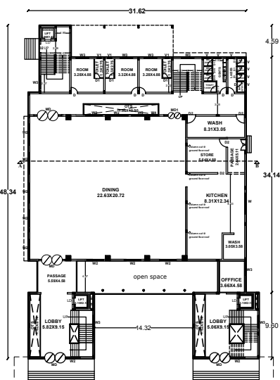
PRO. SECOND FLOOR PLAN
