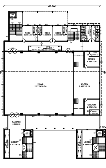
PRO. TERRACE FLOOR PLAN
