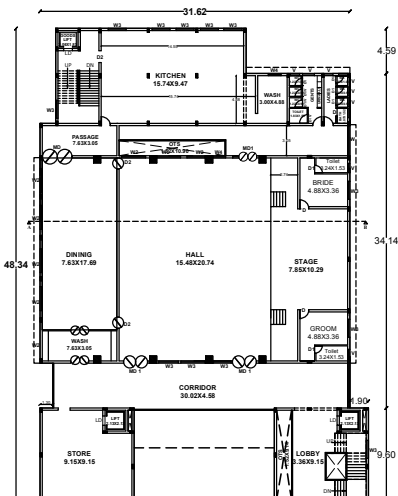
PRO. SECOND FLOOR PLAN
