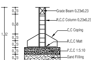
Foundation Detail
