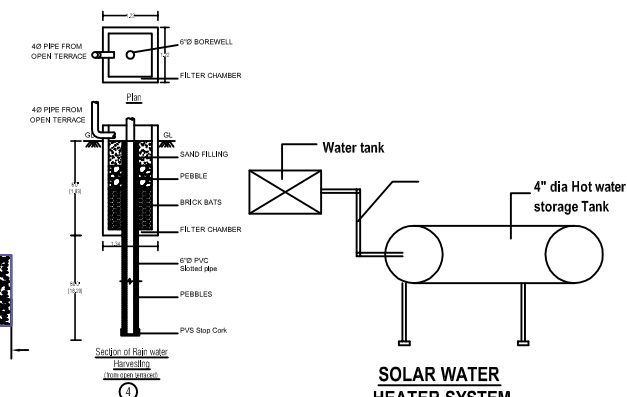
RAINWATER HARVESTING
