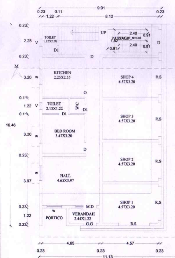
EXI-GROUND FLOOR PLAN
