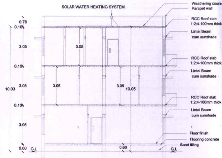
SECTION ON MK
