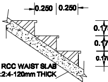
STAIR CASE STEPS SCALE 1:25
