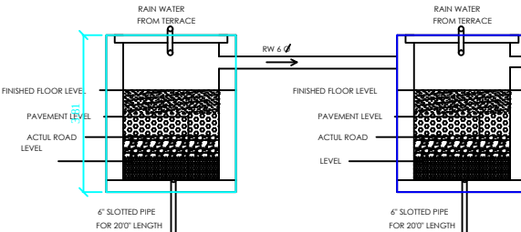
RAINWATER PERCOLATION BED
