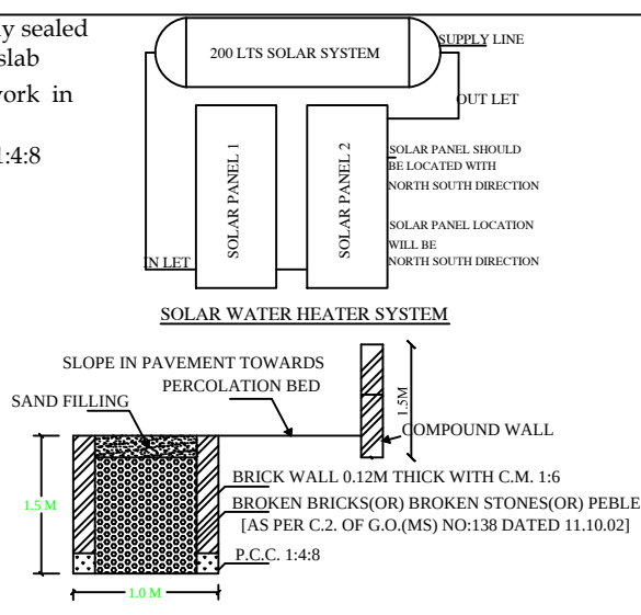
SOLAR WATER HEATER SYSTEM
