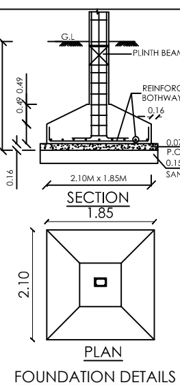
FOUNDATION DETAILS
