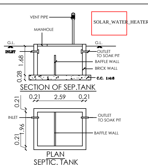
SECTION OF SEP. TANK
