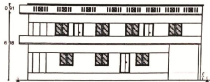
FRONT ELEVATION
