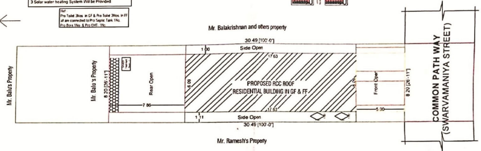
SITE PLAN
