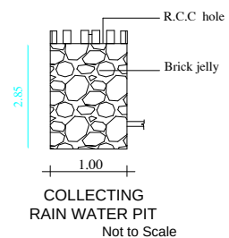
RWHT CAPACITY L=1000 LTRS
