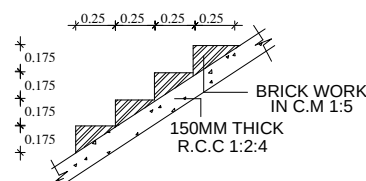
STAIRCASE DETAILS NOT TO SCALE
