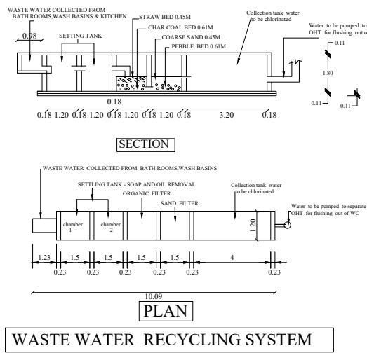
WASTE WATER RECYCLING SYSTEM
