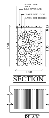
RAIN WATER HARVESTING PERCOLATION BED
