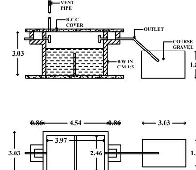
SEPTIC TANK & D-TRENCH DETAILS [NOT TO SCALE]
