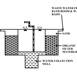
PLAN AND SECTION OF ORGANIC FILTRATION SUMP WITH COLLECTION WELL
