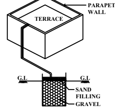
COLLECTION SUMP FOR HARVESTING FOR TERRACE
