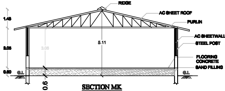
SECTION MK
