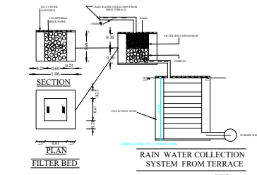
RAIN WATER COLLECTION SYSTEM FROM TERRACE
