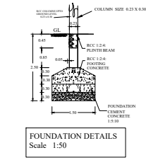
FOUNDATION DETAILS Scale 1:50
