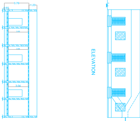
CROSS SECTION ON 'A B'
