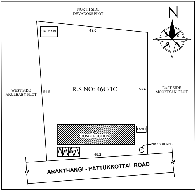
SITE PLAN
