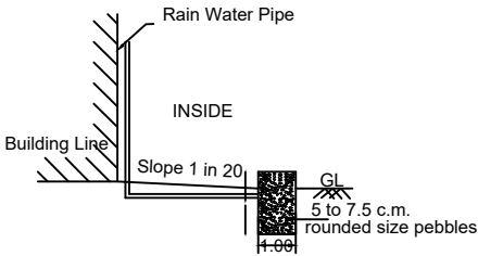
RAINWATER HARVESTING
