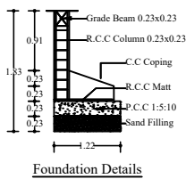
Foundation Details
