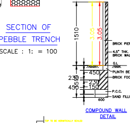
RWH SECTION (SAMPLE)
