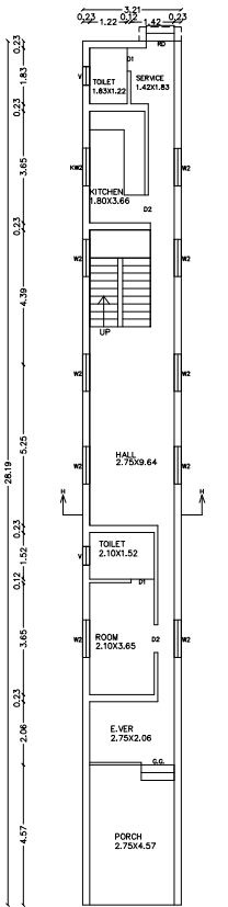
GROUND FLOOR PLAN
