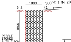
SECTION OF PEBBLE TRENCH SCALE : 1 : = 100
