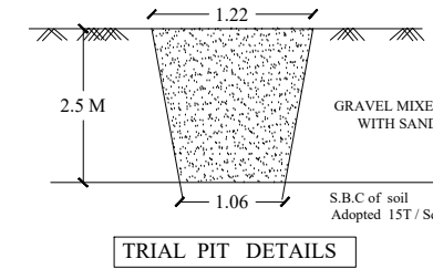
TRIAL PIT DETAILS
