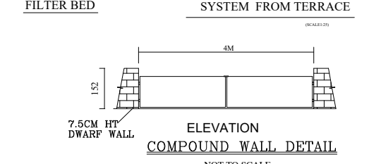
COMPOUND WALL DETAIL
