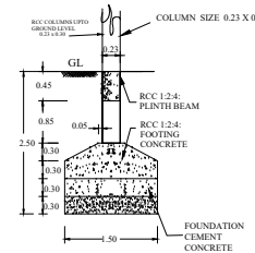
FOUNDATION DETAILS
