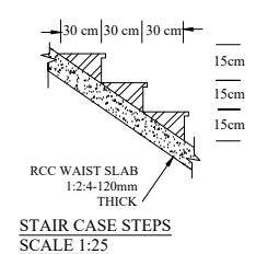
STAIR CASE STEPS SCALE 1:25
