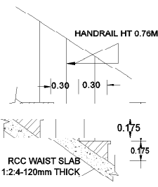
STAIR CASE STEPS SCALE 1:25
