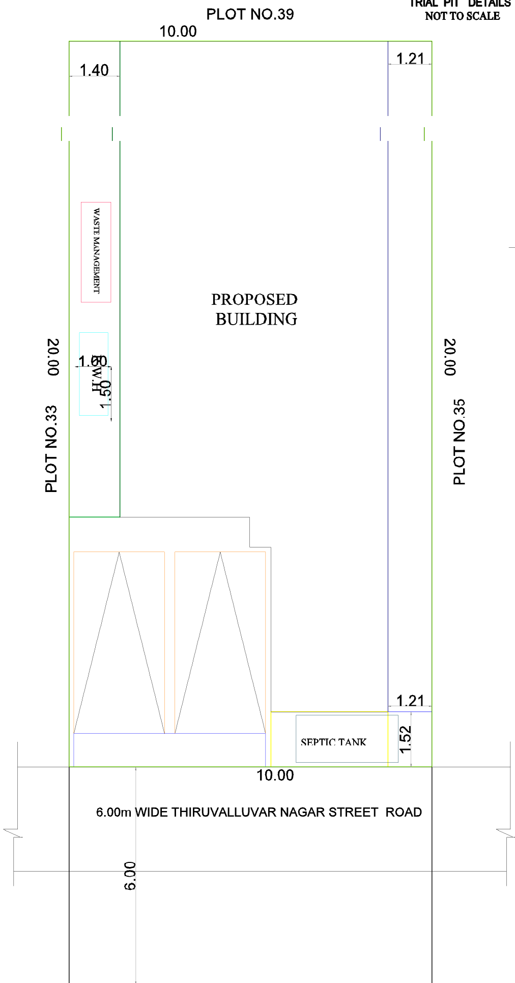
SITE PLAN
