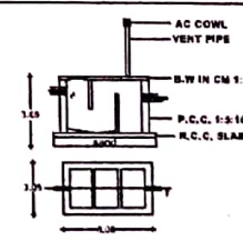
Septic tank detail
