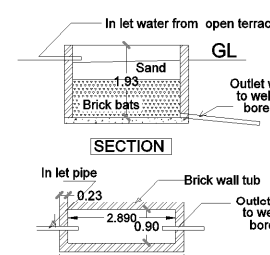
RAIN WATER HARVESTING TANK SCALE 1:25
