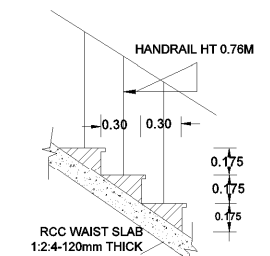
STAIR CASE STEPS SCALE 1:25
