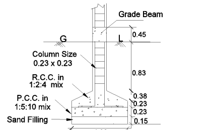
COLUMN DETAILS NOT TO SCALE
