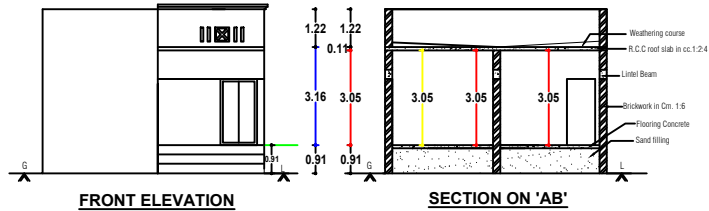
FRONT ELEVATION
