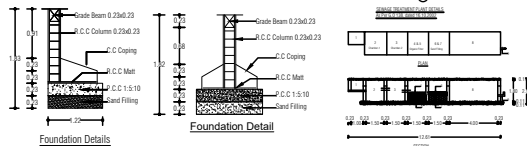
Foundation Details
