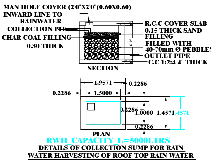
MAN HOLE COVER (75X75) (0.60X0.60)
