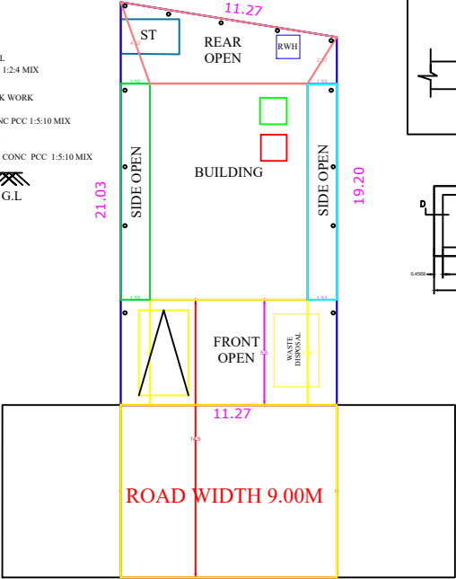
SITE PLAN
