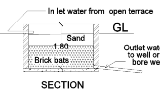
RAIN WATER HARVESTING TANK NOT TO SCALE
