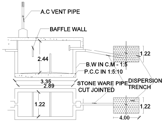
SEPTIC TANK DETAILS NOT TO SCALE
