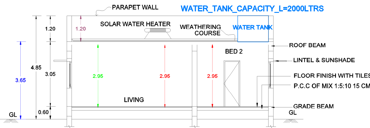
SECTION - BB SECTION
