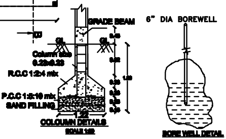
BORE WELL DETAIL
