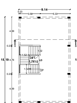
STILT FLOOR PLAN
