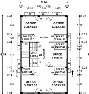
FIRST, SECOND & THIRD FLOOR PLAN
