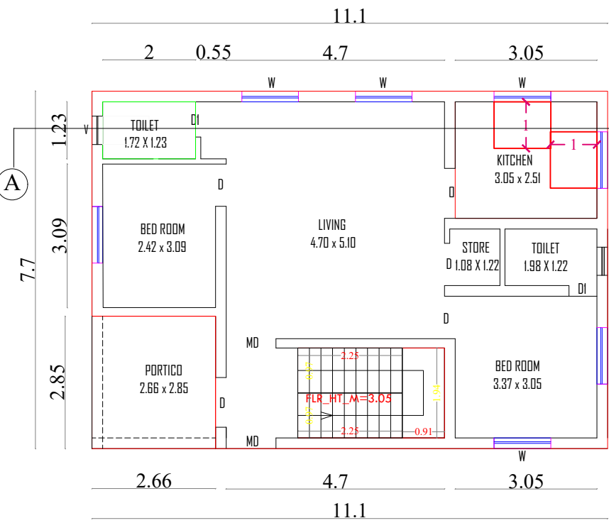
EXISTING & PROPOSED GROUND FLOOR PLAN
