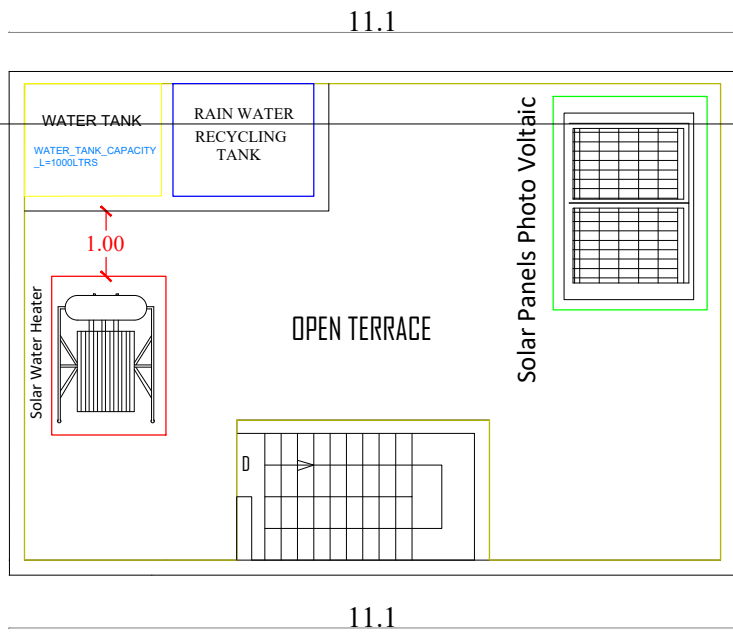
PRO. TERRACE FLOOR PLAN
