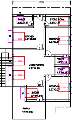
EXT. GROUND FLOOR PLAN
