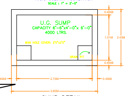
SUMP DETAIL SCALE 1" = 4'-0"
