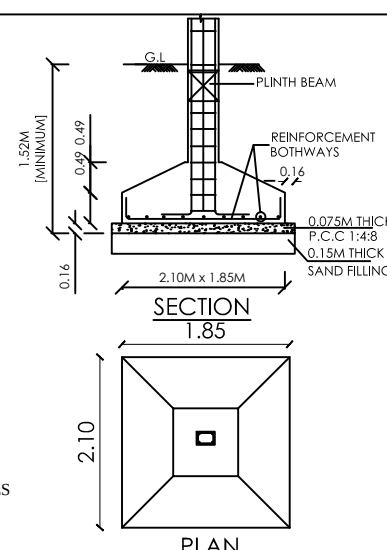
FOUNDATION DETAILS
