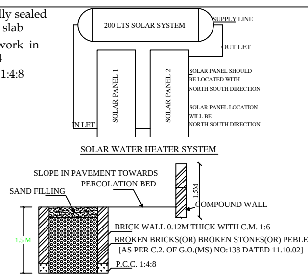
SECTION OF RAIN WATER PERCOLATION BED
