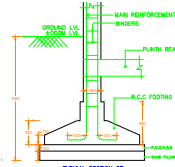
TYPICAL SECTION OF R.C.C COLUMN FOUNDATION SCALE: 1"=1'-0"
