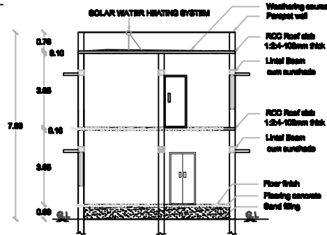
SECTION ON MK
