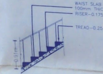
EX-STAIR CASE DETAIL SCALE - 1:50
