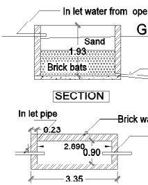
RAIN WATER HARVESTING TANK
