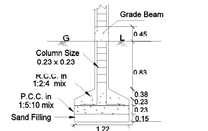
COLUMN DETAILS NOT TO SCALE
