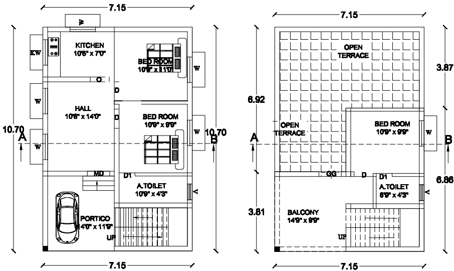
PRO. GROUND FLOOR
