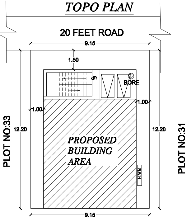
PLOT NO:47 SITE PLAN SCALE (1:100)
