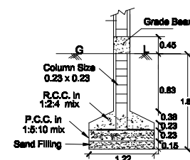
COLUMN DETAILS NOT TO SCALE
