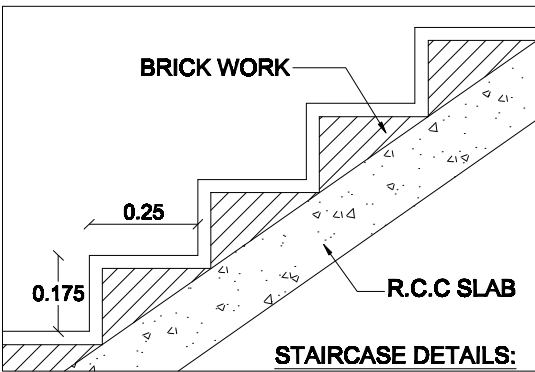
STAIRCASE DETAILS:
