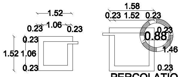
DETAILS OF FILTER BED & SUMP
