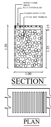
RAIN WATER HARVESTING PERCOLATION BED
