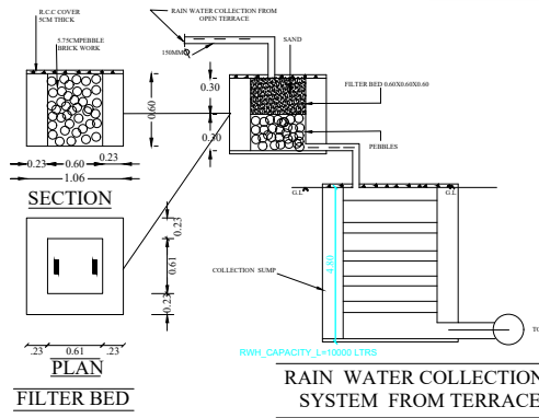
RAIN WATER HARVESTING PERCOLATION BED
