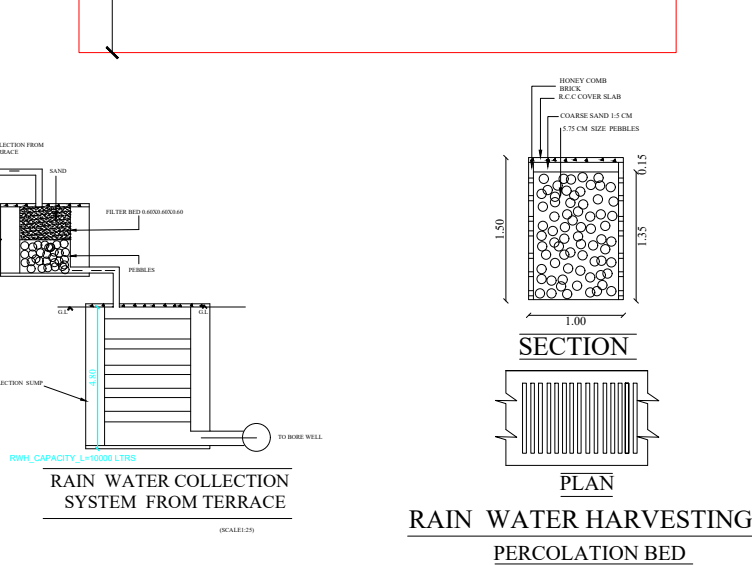
FILTER BED
