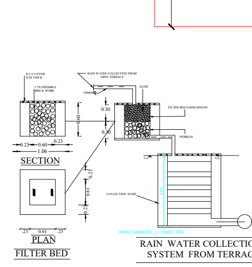
FILTER BED
