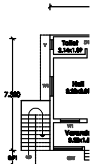
EXI.GROUND FLOOR PLAN
