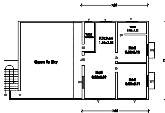
PRO.FIRST FLOOR PLAN
