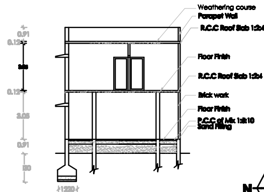
SECTION ON "PQ"
