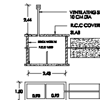
SEPTIC TANK DETAIL
