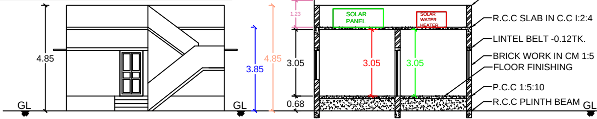
FRONT ELEVATION
