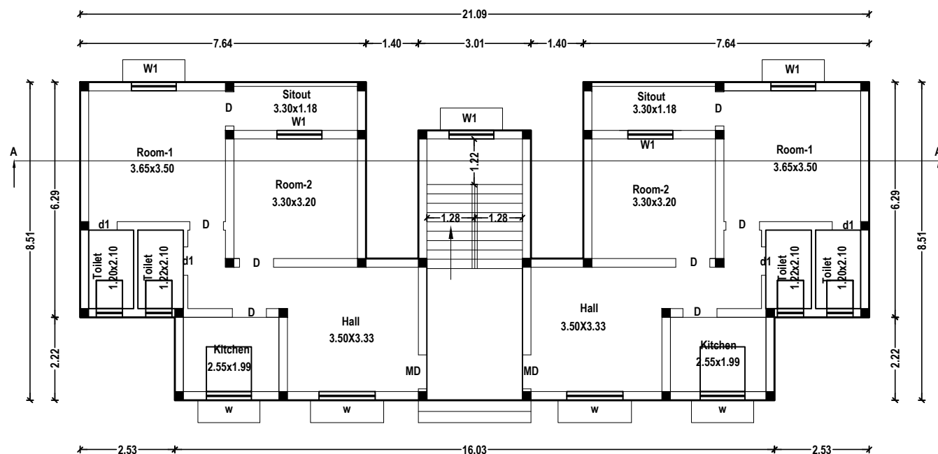
GROUND FLOOR STAFF QUARTERS
