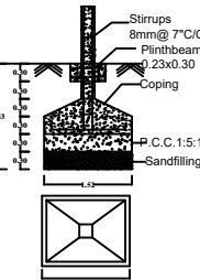
Foundation Details
