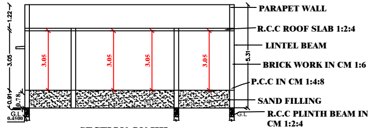
SECTION ON HH
