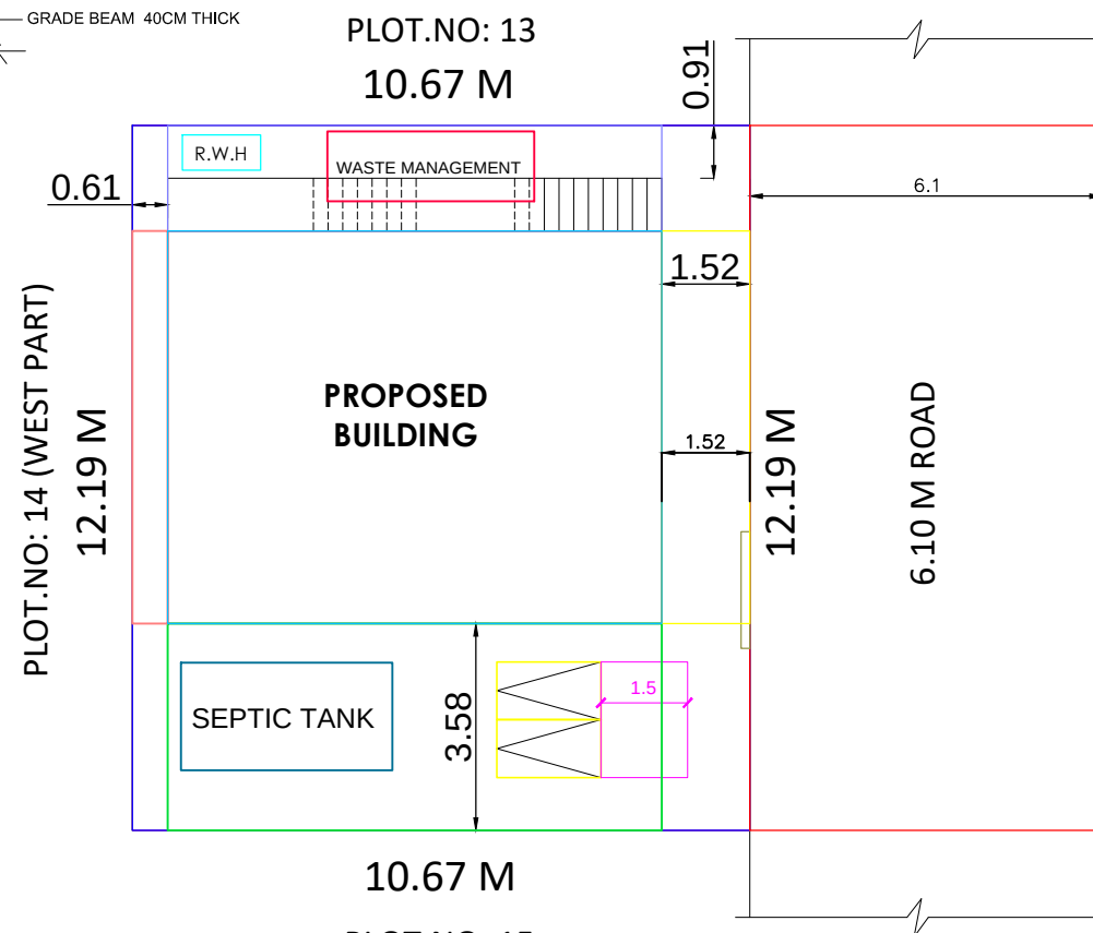
SITE PLAN
