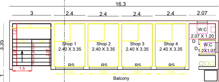
PRO. TERRACE FLOOR PLAN
