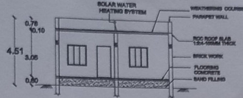
SECTION ON RM
