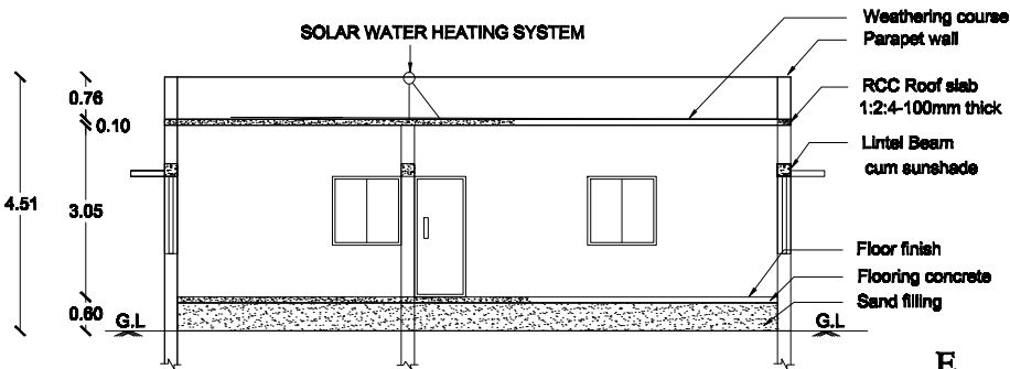
SECTION ON MK
