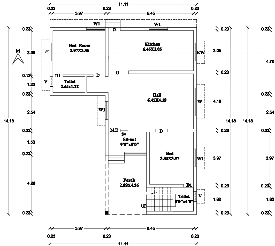
PRO-GROUND FLOOR PLAN
