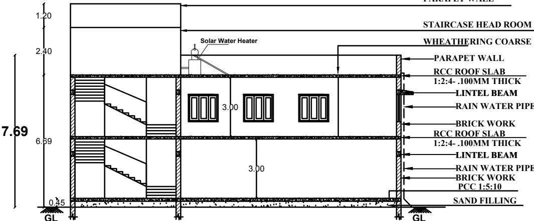
SECTION - A B
