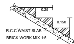
STAIRCASE DETAIL
