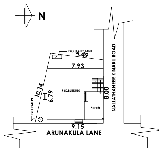
SITE PLAN
