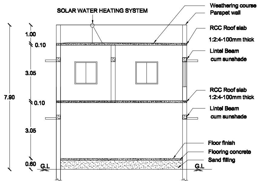
SECTION ON MK
