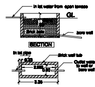
RAIN WATER HARVESTING TANK
