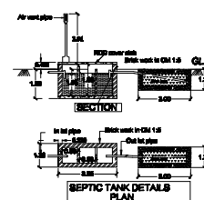
SEPTIC TANK DETAILS PLAN
