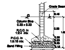
COLUMN DETAILS NOT TO SCALE
