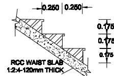
STAIR CASE STEPS SCALE 1:25
